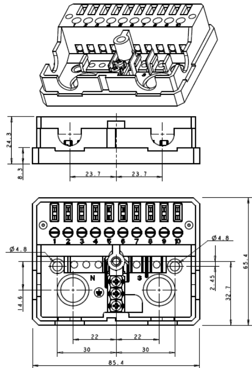
AB Socket
