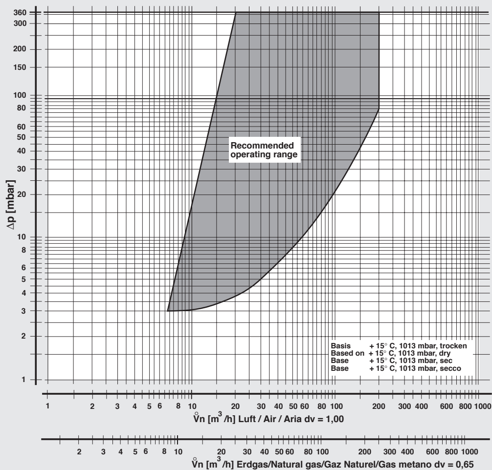
Flow diagram MB-VEF 420 B01 Rp 2, with microfilter
